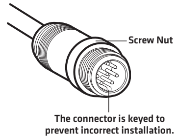
Hand-Tightening the Screw Nut
