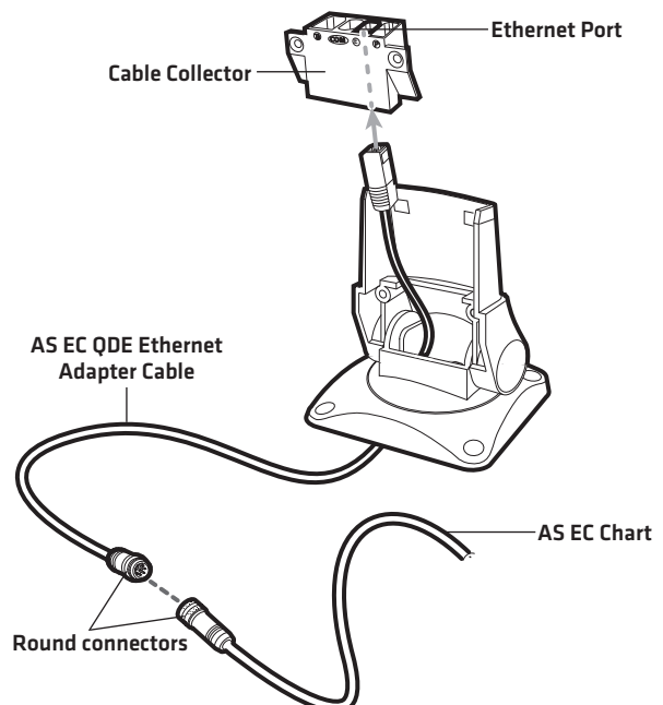
Connecting the Ethernet Cables to a 700 Series HD Unit
